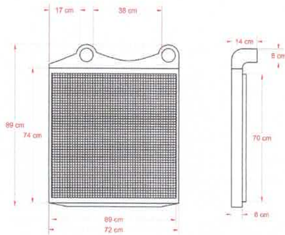
BITON DPP CUMMINS CHARGE AIR COOLER
